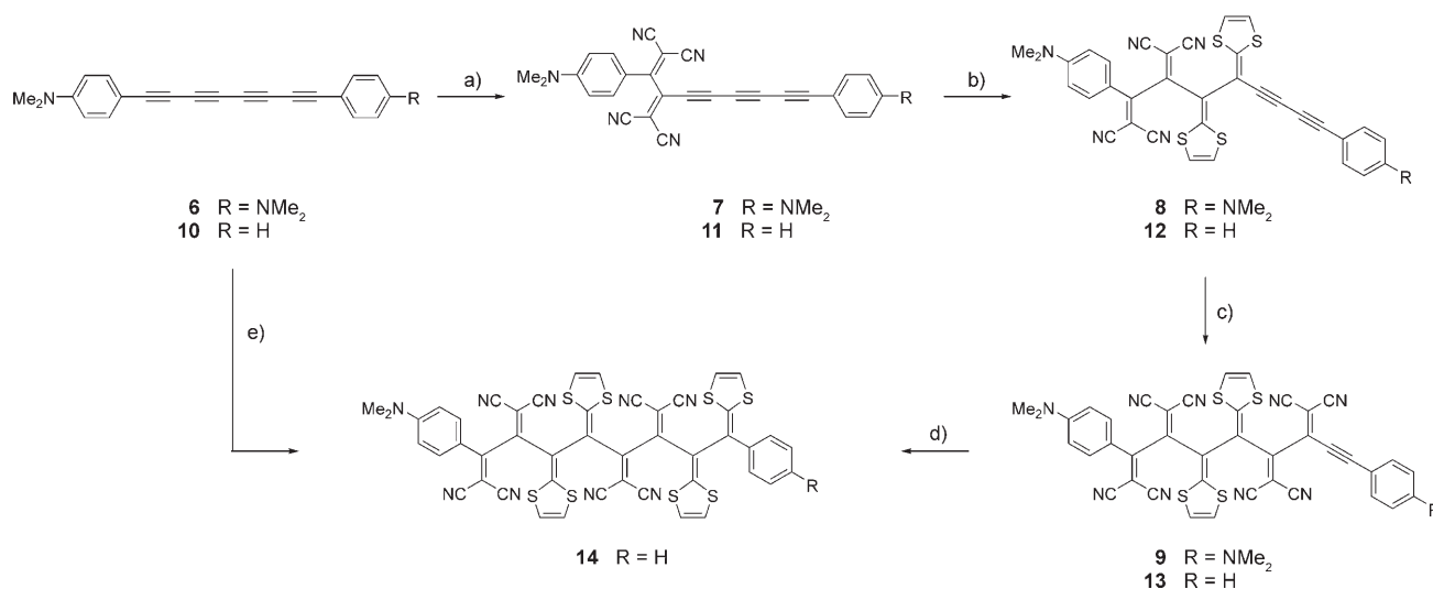
Scheme 1. Cascade of alternating [2+2] cycloadditions/retro-electrocyclizations of TCNE/TTF to octatetraynes 6 and 10 . a) TCNE, \text{CH}_2\text{Cl}_2 , 10–14 h, 20^\circ\text{C} , 72% ( 7 ), 95% ( 11 ). b) TTF, MeCN, 16–17 h, 60^\circ\text{C} , 80% ( 8 ), 78% ( 12 ). c) TCNE, \text{CH}_2\text{Cl}_2 , 14–22 h, 20^\circ\text{C} , 83% ( 9 ), 92% ( 13 ). d) TTF, \text{CH}_2\text{Cl}_2/\text{MeCN} 1:1, 3 h, 50^\circ\text{C} , 21% ( 14 ). e) TCNE, TTF, \text{CH}_2\text{Cl}_2/\text{MeCN} 1:1, 22 h, 50^\circ\text{C} , 21% ( 14 ).
